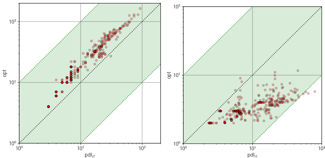
(a) Decision set/list size detailed: pdl_i^{\uparrow} vs. opt (b) Explanation size detailed: pdl_i^{\uparrow} vs. opt
