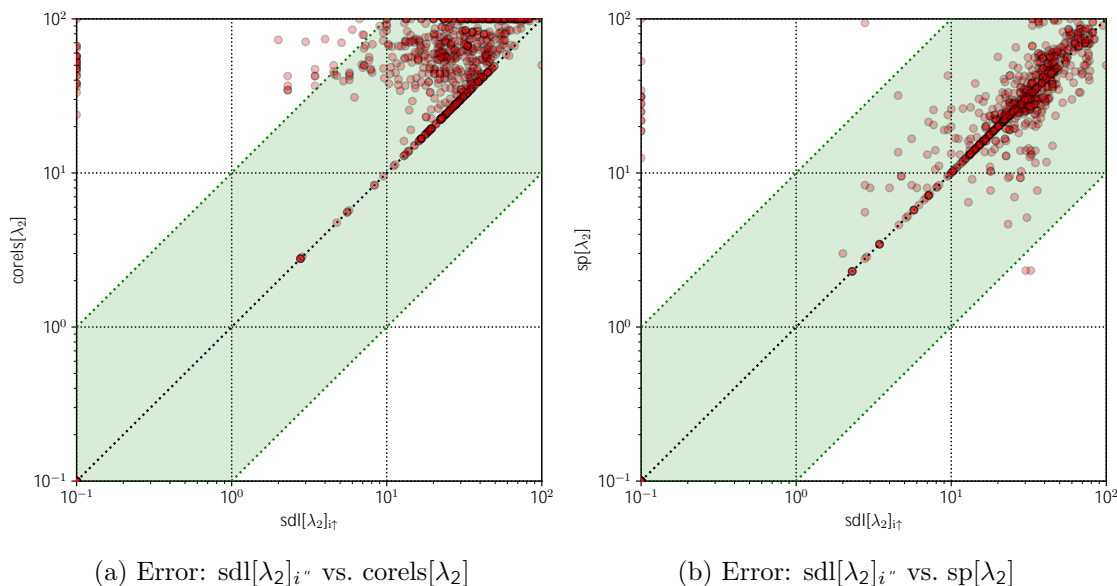
Figure 9: Test error comparison of sdl[\lambda_2]_{i^*} , corels[\lambda_2] , and sp[\lambda_2] .
