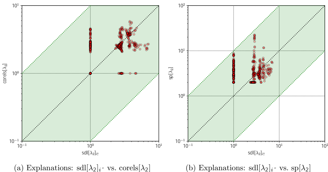
Figure 10: Comparison of sdl[\lambda_2]_{i\uparrow} , cores[\lambda_2] , and sp[\lambda_2] in terms of average explanation size.
